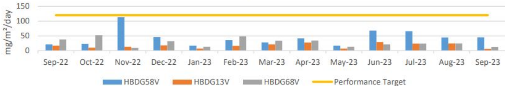
Dust Deposition Total Insoluble Matter Historical Trend Graphs for Dust Sensitive Receptors September 2022 to September 2023
